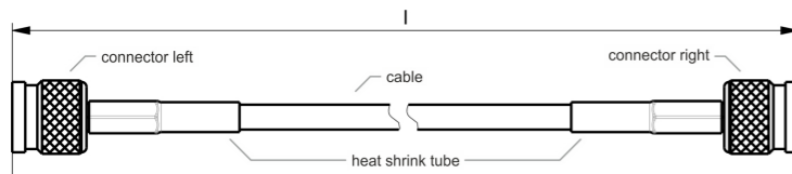
Connecting Cable 52010174/52010175/52010176/52010177
